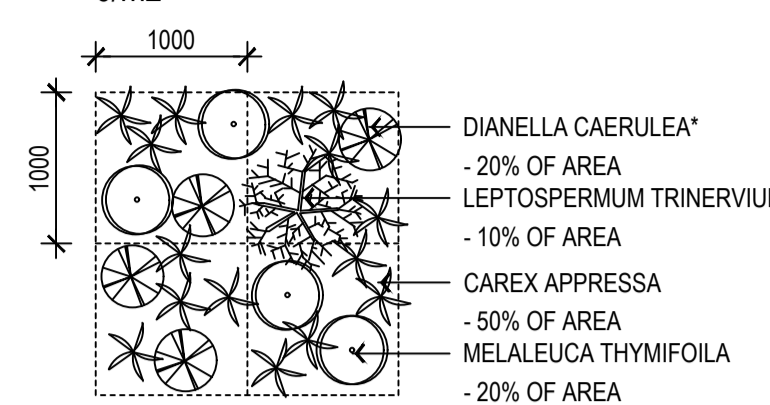
02 DETAIL
