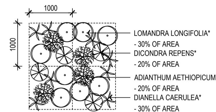
05 DETAIL
